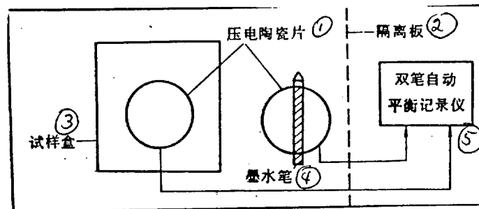
ILLUSTRATION SIX: DIAGRAM OF ARRANGEMENT OF PIEZOELECTRIC CRYSTAL EXPERIMENT
