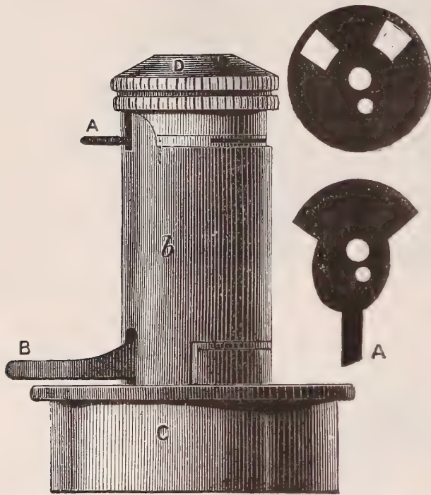
FIG. 209.—Powell and Lealand's chromatic oil condenser.
