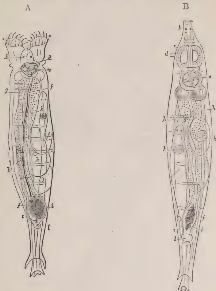
FIG. 542.— Rotifer vulgaris , as seen at B, with the wheels drawn in, and at A with the wheels expanded : b , eye-spots ; c , wheels ; d , antenna ; e , jaws and teeth ; f , alimentary canal ; g , cellular mass inclosing it ; h , longitudinal muscles ; i, i , tubes of water-vascular system ; j , young animal ; l , cloaca.
