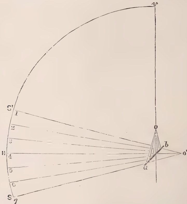
FIG. 305.—Light from the open sky falls upon the mirror in all directions.
