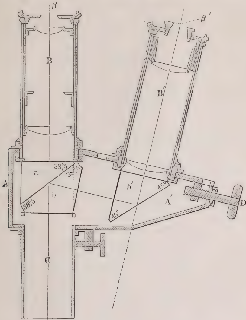
FIG. 82.—Abbe's binocular eye-piece.
