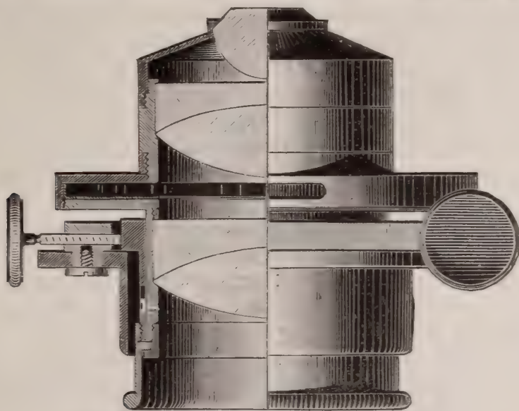
FIG. 211.—Abbe's achromatic condenser.
