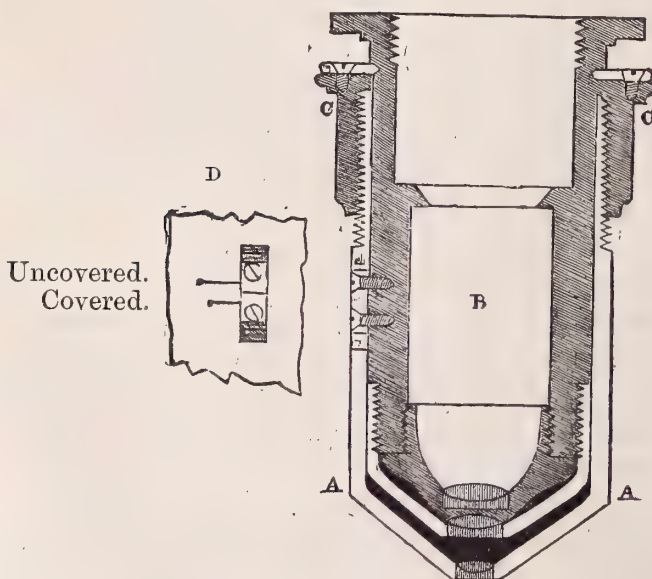
FIG. 270.—Section of adjusting object-glass.
