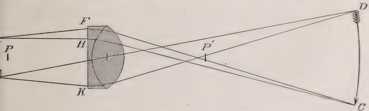
FIG. 26.—The formation of a real image.
