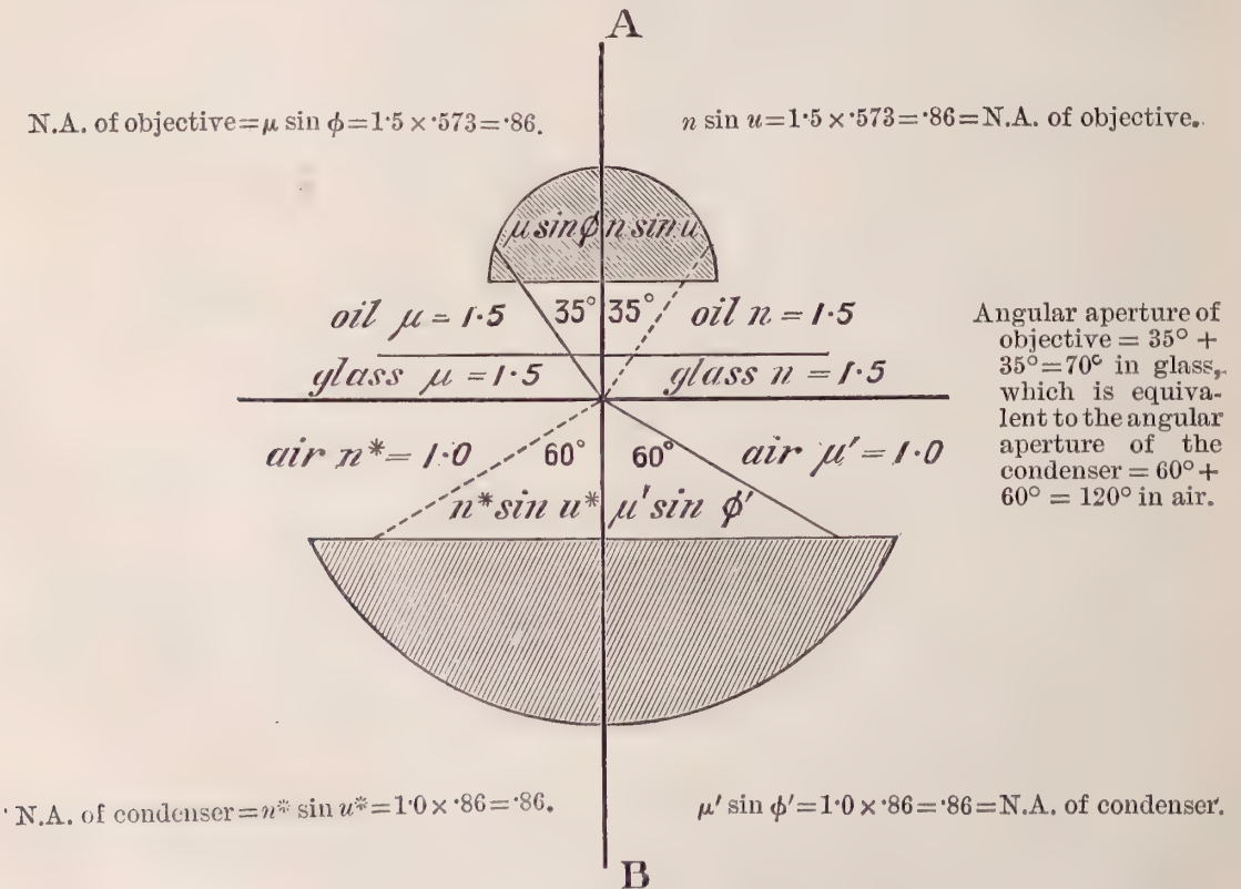
FIG. A1.—Identity of n \sin u (German math. form) with \mu \sin \phi (English). Also N.A. and angular aperture.
