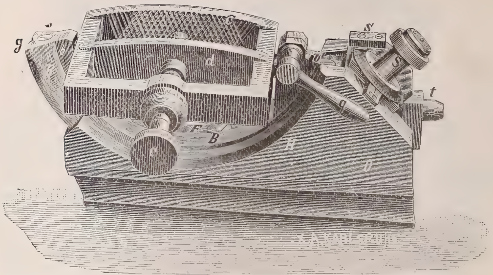
FIG. 348.—Object-holder for analysis by diversified section.
