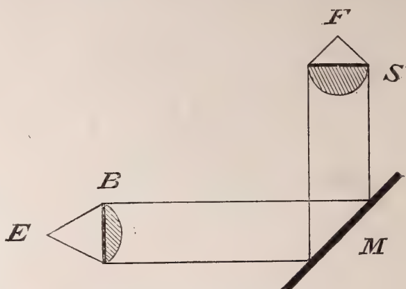
FIG. 308.—Illumination for dark ground (with stop beneath the condenser).
