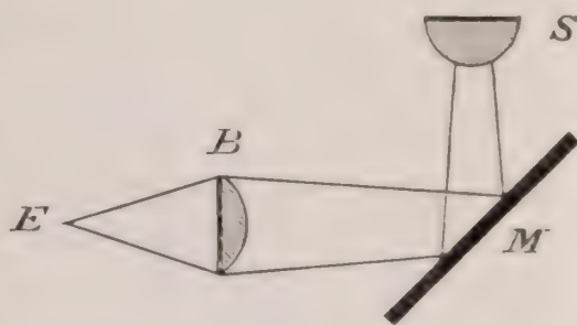
FIG. 311.—Absurdity of using a bull's-eye with the edge of the lamp flame not in its principal focus.
