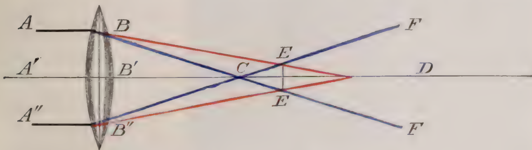
FIG. 19.—Chromatic aberration.
