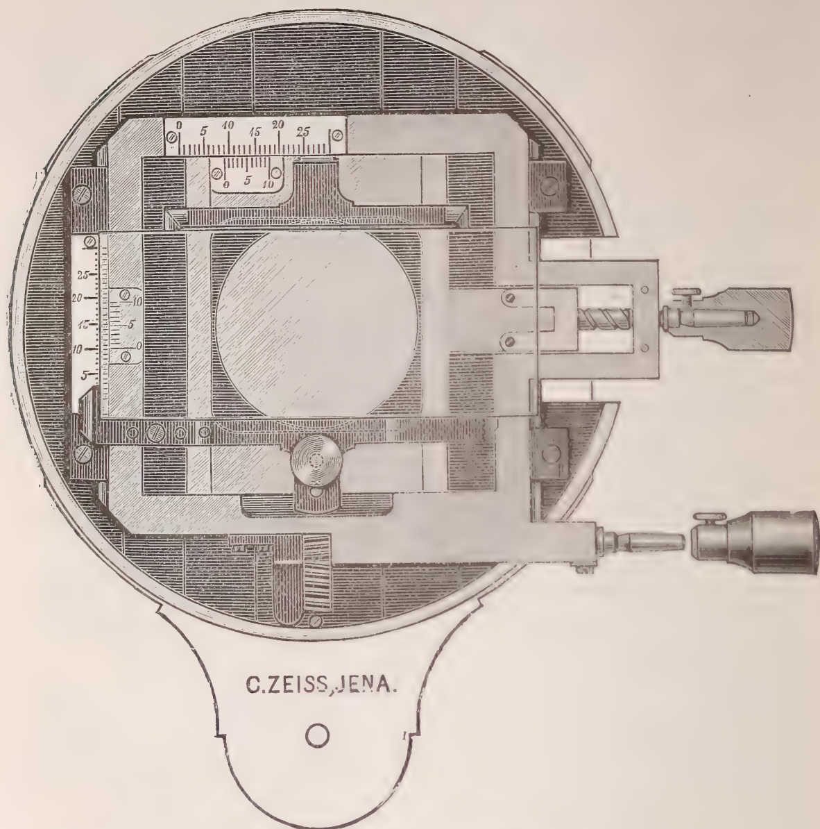
FIG. 128 A.—Zeiss's mechanical stage.
