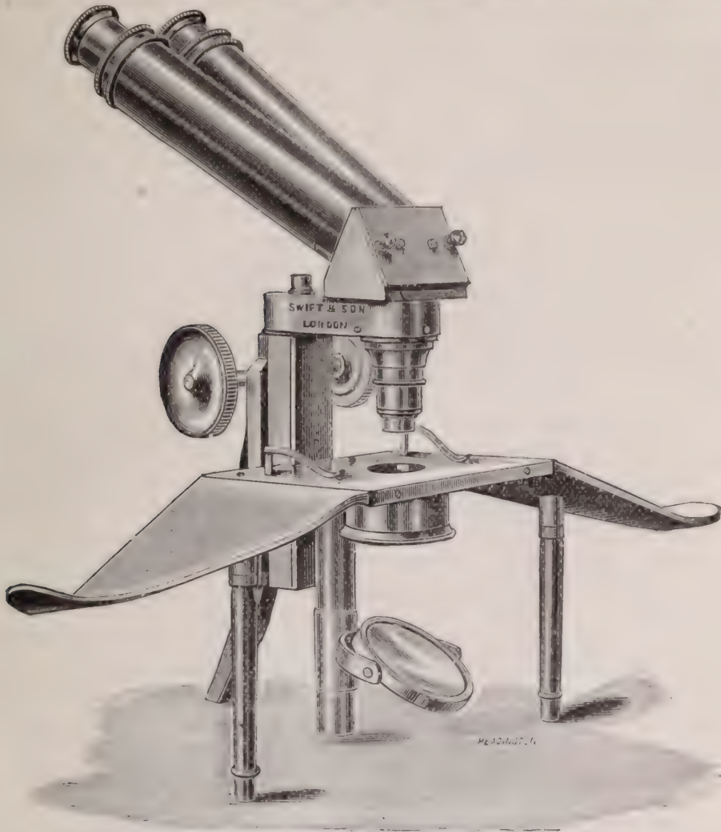
FIG. 338.—Swift's Stephenson binocular dissecting microscope.
