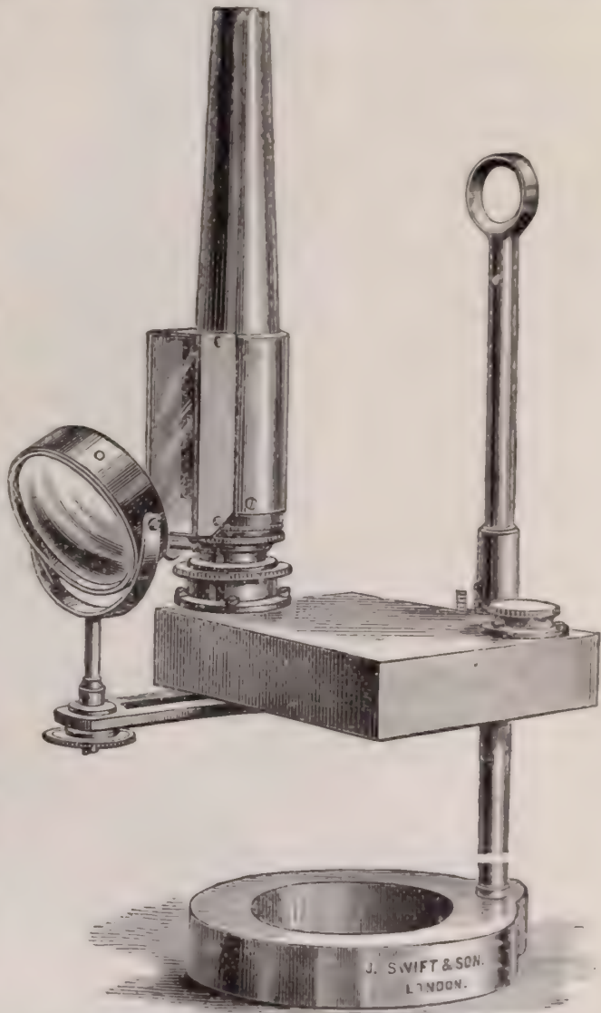
FIG. 293.—Lamp devised by Mr. E. M. Nelson.
