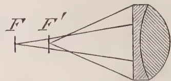
FIG. 23.—Under-corrected system.
