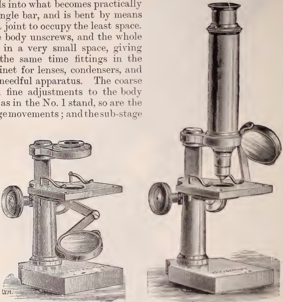
FIG. 152.—Beck's histological and dissecting microscope.
