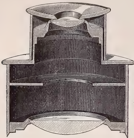
FIG. 278.—Huyghenian eye-piece.
