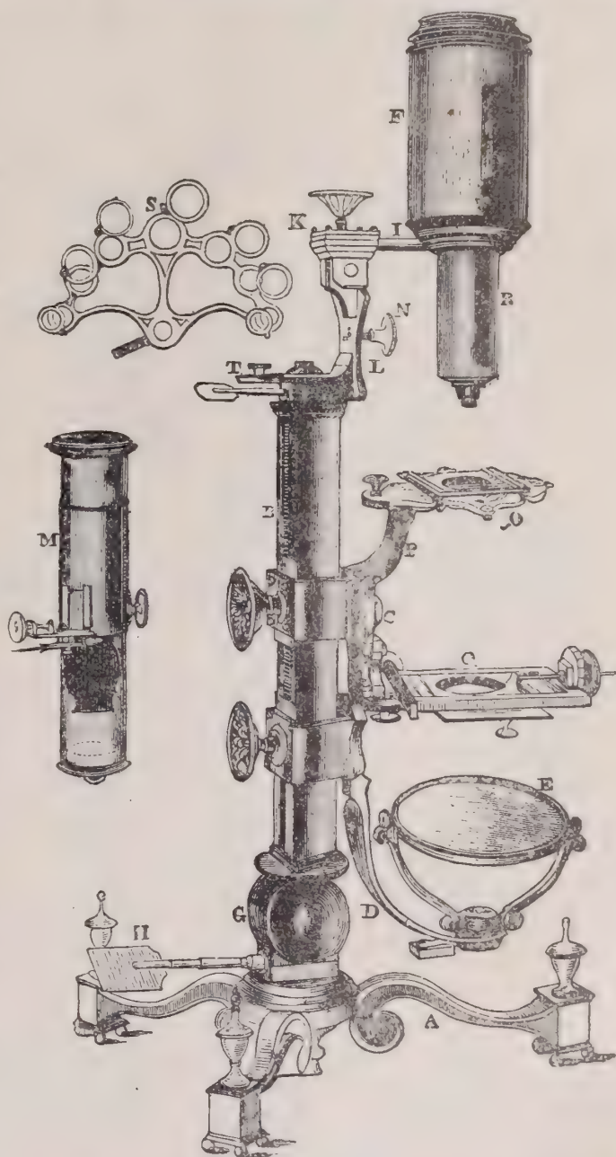
FIG. 106.—Martin's large universal microscope as used by Quekett.
