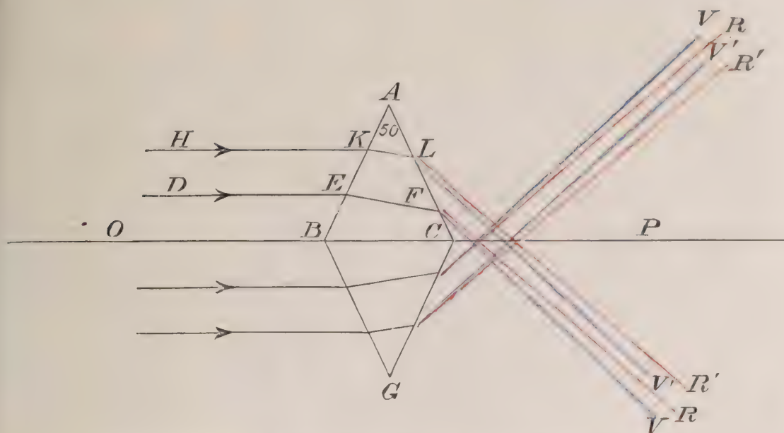
FIG. 8.—Action of a pair of prisms with their bases in contact on parallel light.
