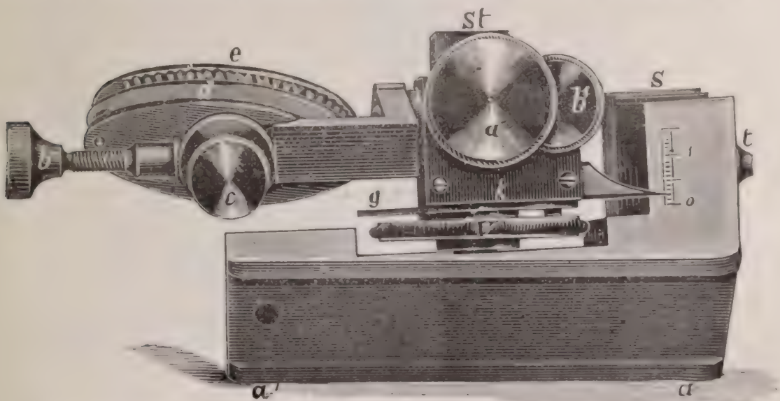
FIG. 347.—Object-holder movable about two horizontal axes at right angles to each other.
