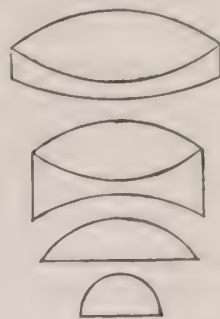
FIG. 275.—Combination for 'homogeneous' immersion by Abbe.
