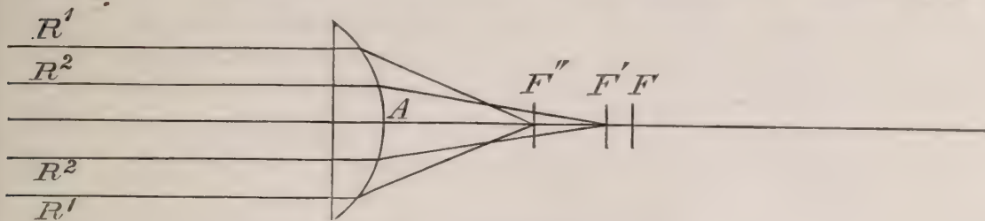
FIG. 17.—Spherical aberration.
