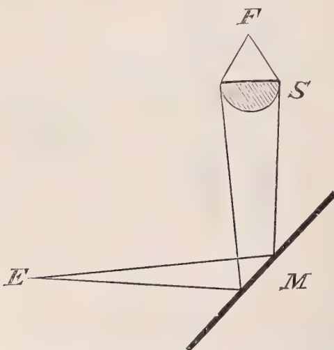
FIG. 300.—Another method of getting critical image.
