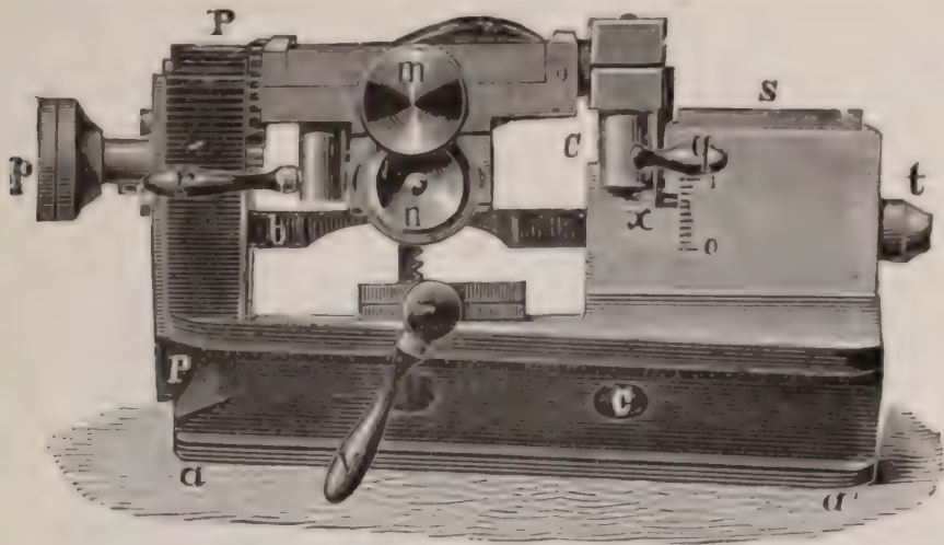
FIG. 346.—Object-holder with jaws.
