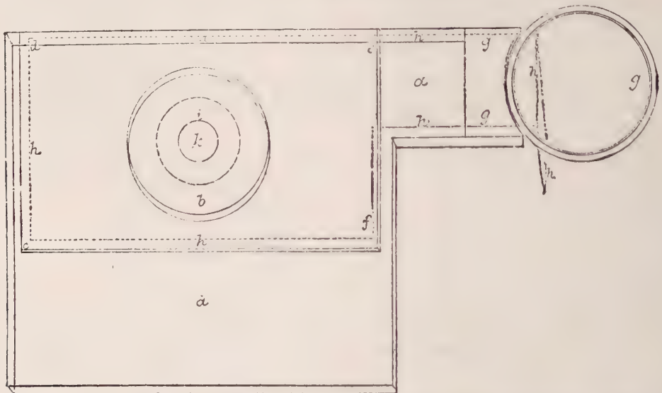
FIG. 250.—Dallinger and Drysdale's moist continuous growing stage.
