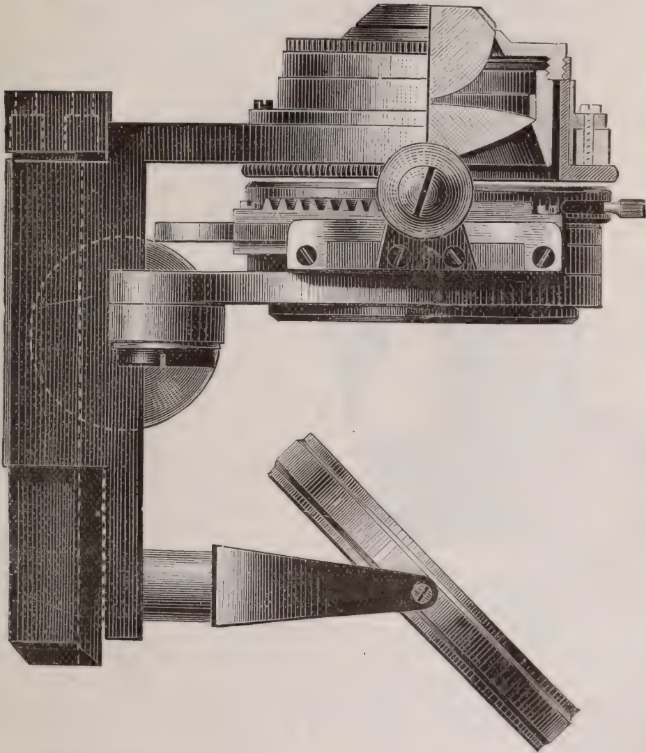
FIG. 208.—Abbe's chromatic condenser as applied to the Zeiss microscopes.
