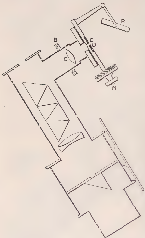
FIG. 227.—Bright-line spectro-micrometer.
