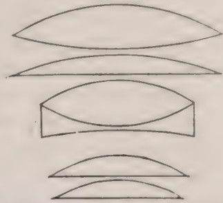
FIG. 274.—A suggested combination by Wenham, 1869.
