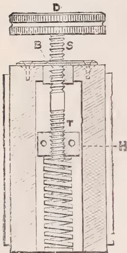
FIG. 127.—Campbell's differential screw fine adjustment.
