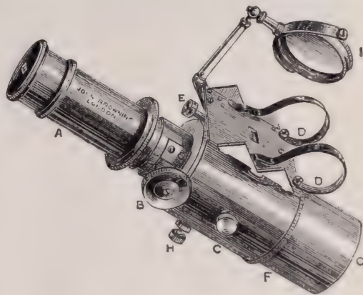
FIG. 225.—Micro-spectroscope.
