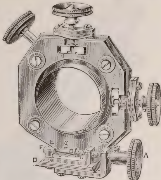
FIG. 130.—Powell and Lealand's sub-stage with fine adjustment.
