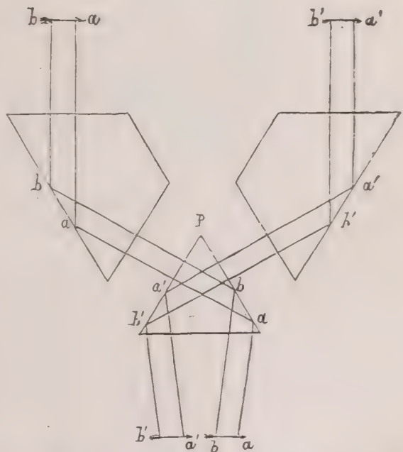
FIG. 73.—Arrangement of prisms in Nacht's stereoscopic binocular microscope.
