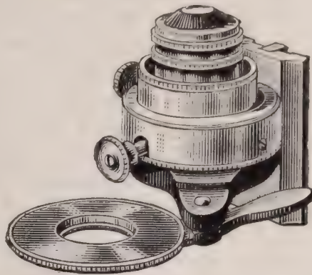
FIG. 147.—Centring nose-piece used as sub-stage.
