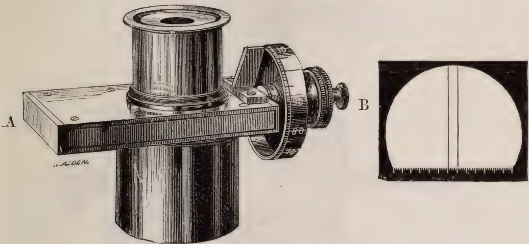
FIG. 175.—The micrometer eye-piece.
