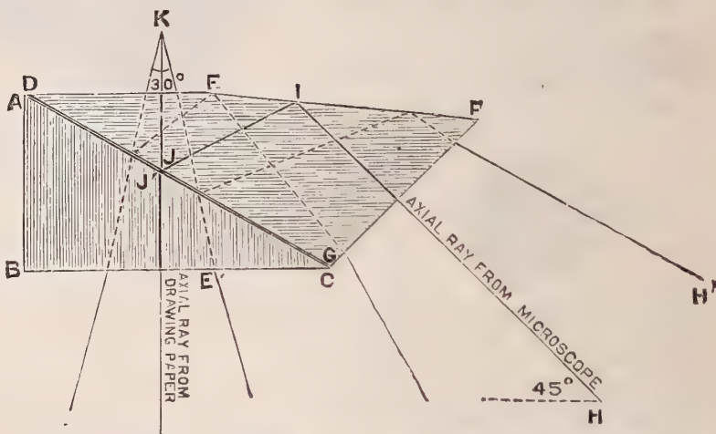
FIG. 185.—Diagram explaining Schröder's camera lucida.
