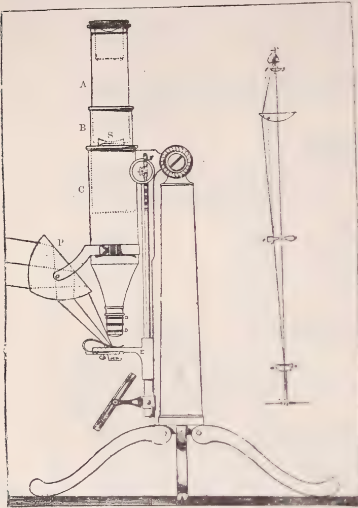
FIG. 111.—Sellique's achromatic microscope (1823-4).
