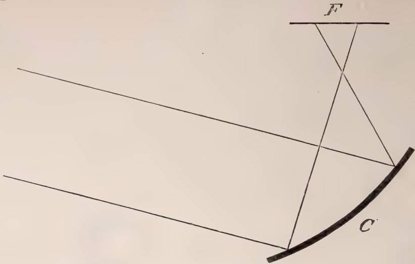
FIG. 304.—Erroneous method of arrangement for 'diffused daylight.'
