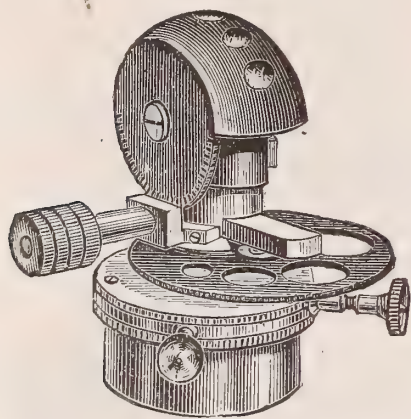
FIG. 213.—Beck's variable condenser.
