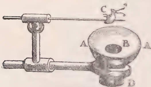
FIG. 105.—Lieberkuhn's microscope.
