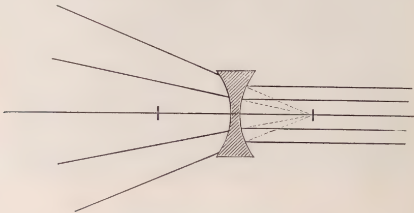
FIG. 16.—‘Virtual’ focus of concave lens.
