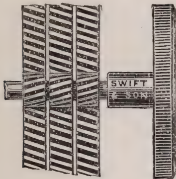
FIG. 119.—'Stepped' diagonal rack-work for coarse adjustment.
