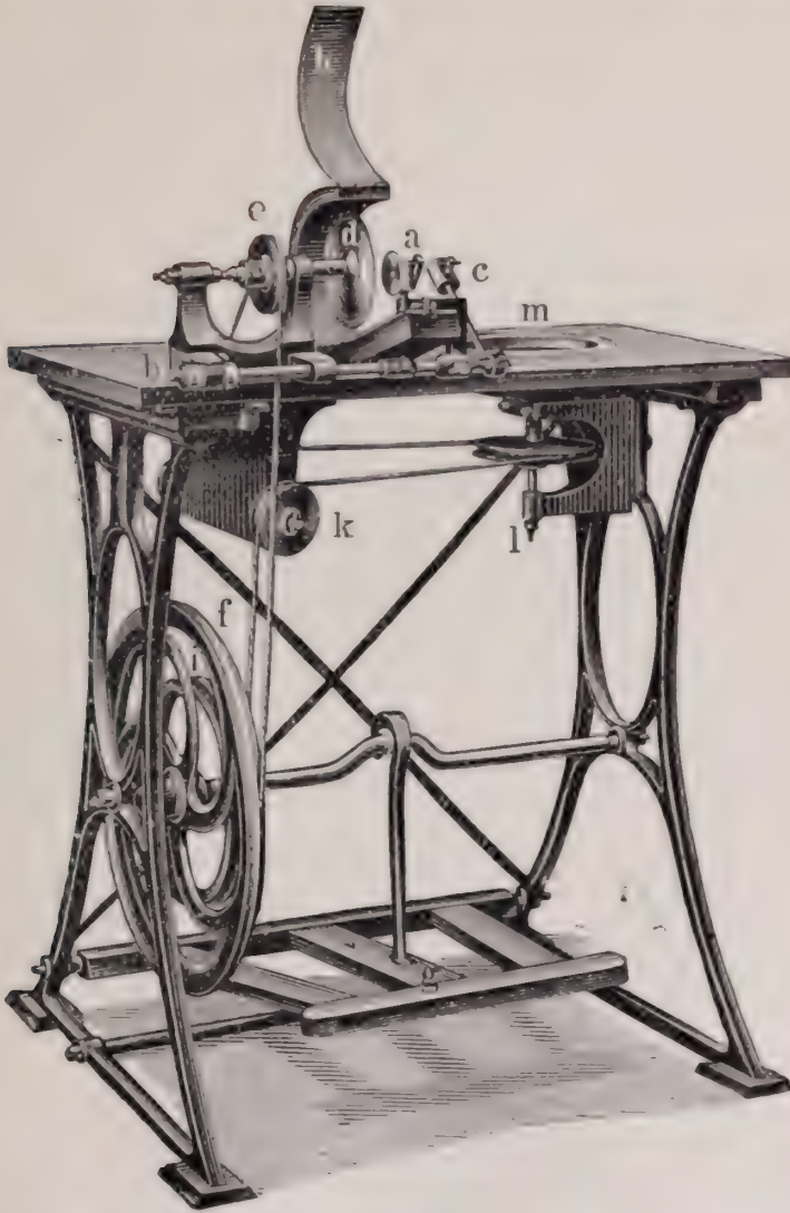
FIG. 359.—Treadle machine for cutting hard sections.
