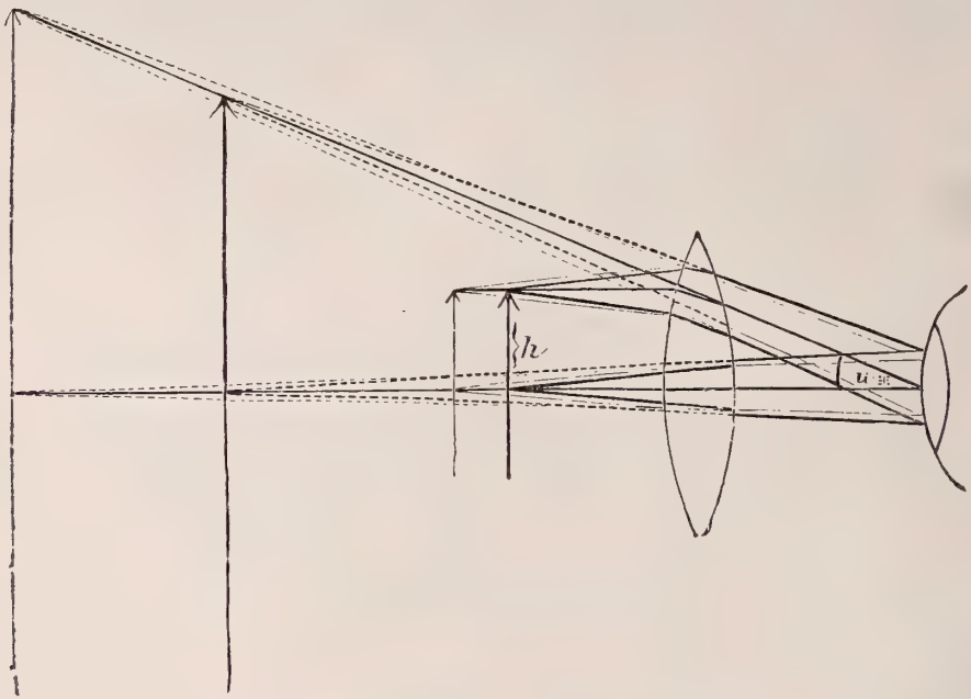
FIG. 28.—The amplifying power of a lens.
