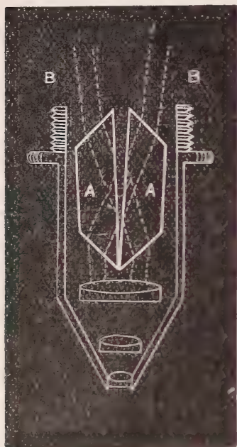
FIG. 77.—Riddell's binocular prisms, as applied by Mr. Stephenson.
