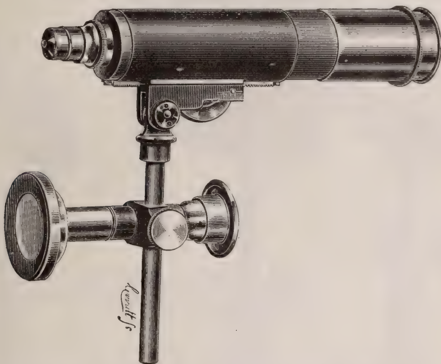
FIG. 171.—Collins's aquarium microscope, applied to the aquarium by a 'sucker.'
