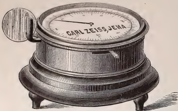
FIG. 325.—Zeiss's cover-glass tester.
