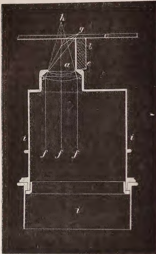
FIG. 216.—Wenham's reflex illuminator.
