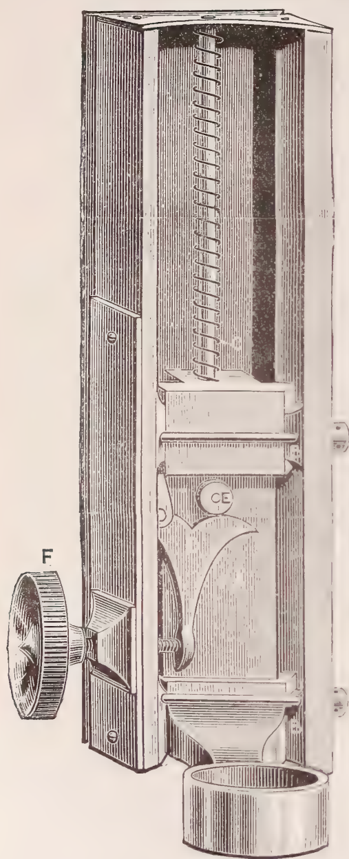
FIG. 124.—Swift's patent fine adjustment.
