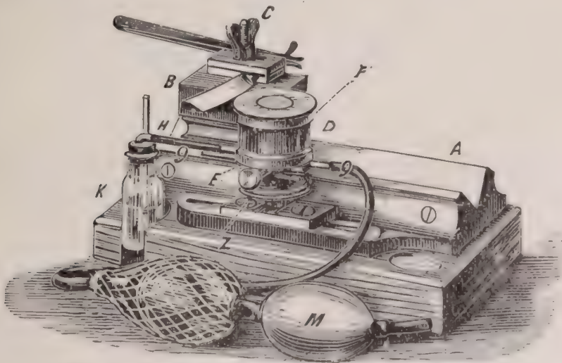
FIG. 354.—Dr. Hayes's ether freezing microtome.
