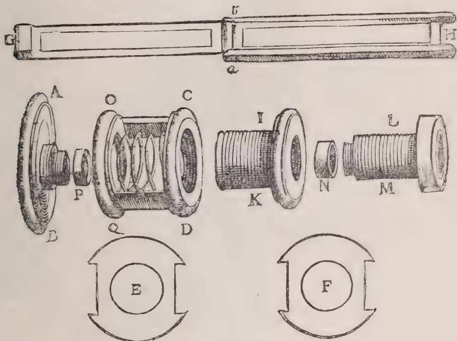
FIG. 102.—Hartsoeker's simple microscope (1694).
