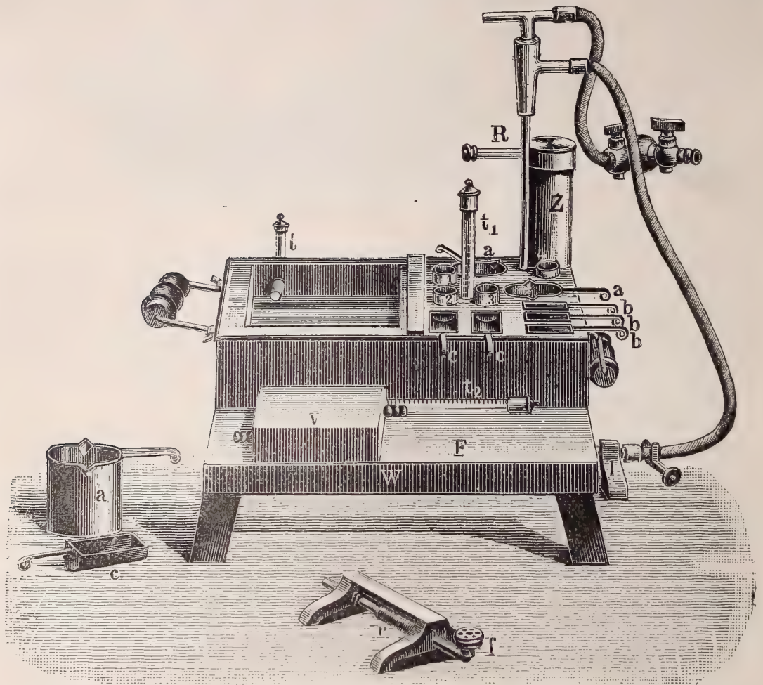
FIG. 333.—Apparatus for preparing mounting media, paraffin, &c. for imbedding by heat.
