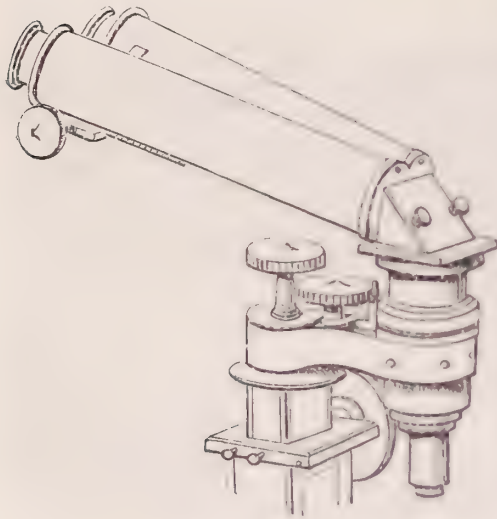
FIG. 81.—Stephenson's erecting binocular.
