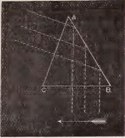
FIG. 80.—Stephenson's erecting prism.
