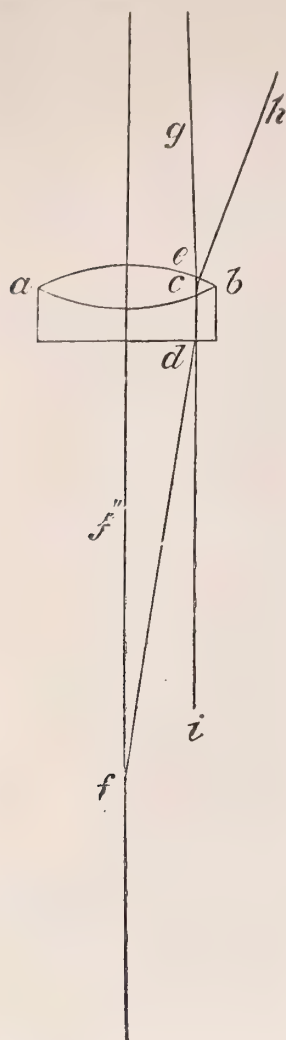
FIG. 268.—The two aplanatic foci of an optical combination.
