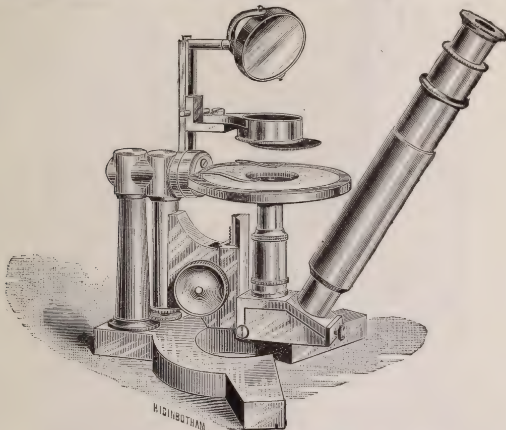
FIG. 167.—The 'University' microscope as a chemical instrument.
