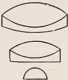
FIG. 273.—A single-front combination by Wenham.
