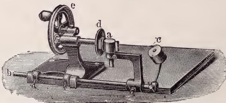
FIG. 358.—Hand machine for cutting hard sections.
