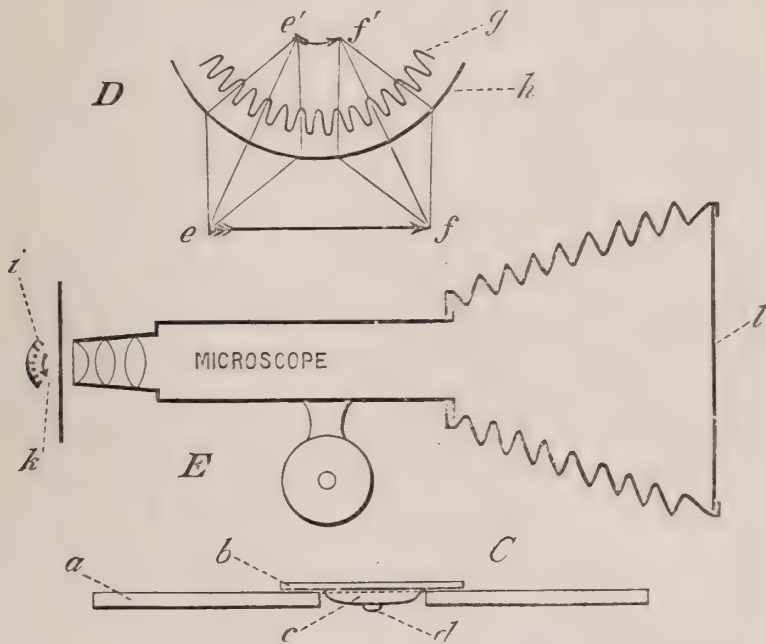
FIG. 675B.—Diagrammatic illustration of the method by which the image in fig. 675A was photo-micrographed.
