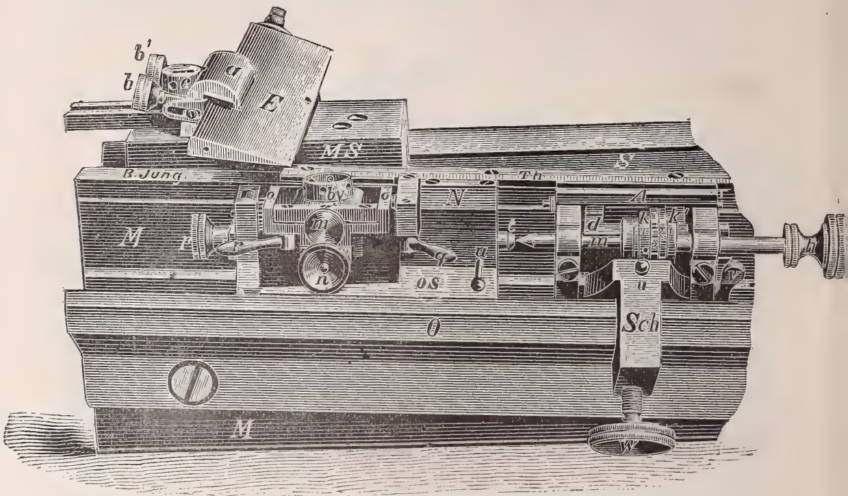
FIG. 345.—The Thoma microtome with special knife.
