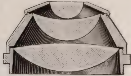
FIG. 207.—Optical arrangement of Abbe's chromatic condenser.
