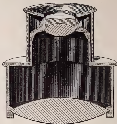
FIG. 279.—Kellner eye-piece.
