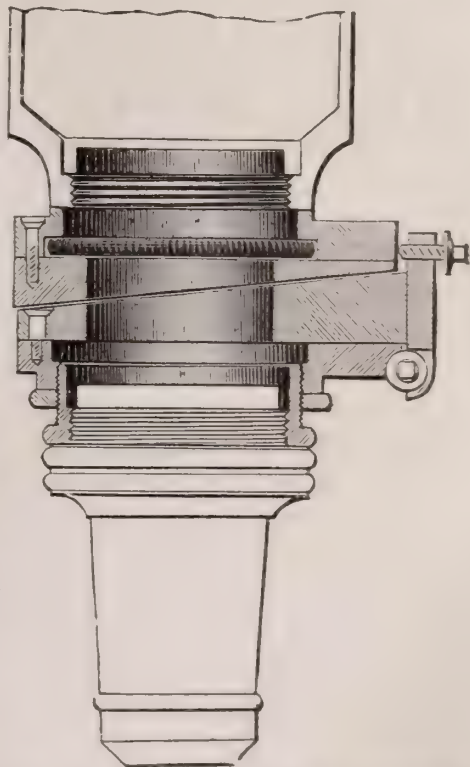
FIG. 193.—Zeiss's sliding-objective changer, with objective in position.
