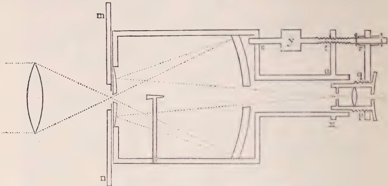
FIG. 109.—Smith's reflecting microscope (1738).
