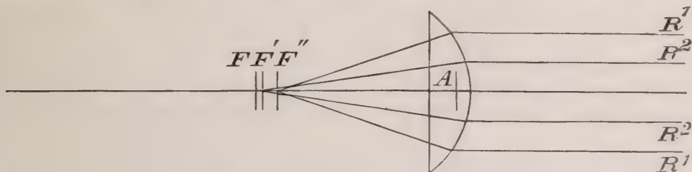
FIG. 18.—Spherical aberration.
