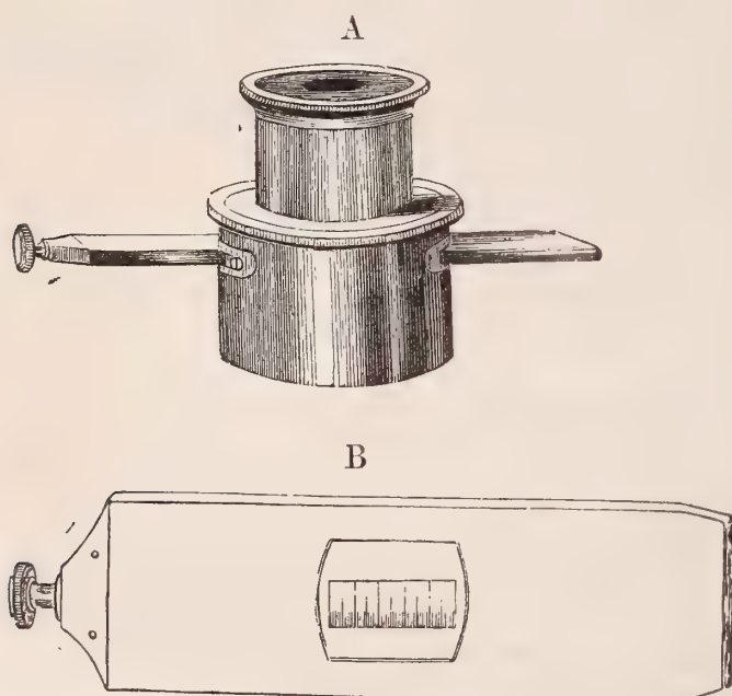
FIG. 178.—Jackson's eye-piece micrometer.
