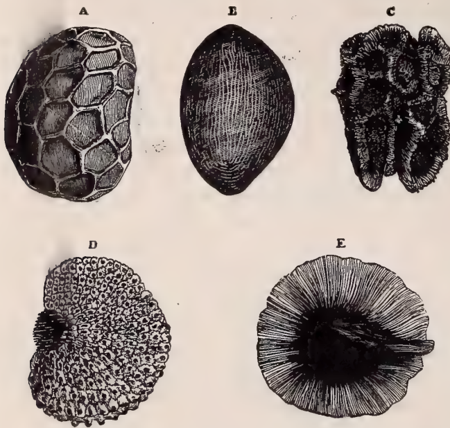
FIG. 508.—Seeds as seen under a low magnifying power: A, poppy; B, Amaranthus (prince's feather); C, Antirrhinum majus (snapdragon); D, Dianthus (clove-pink); E, Bignonia .
