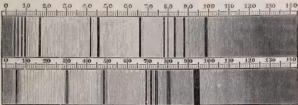
FIG. 228.—Upper half, map of solar spectrum, showing Fraunhofer lines. Lower half, absorption spectrum, showing position of bands in relation to lines.
