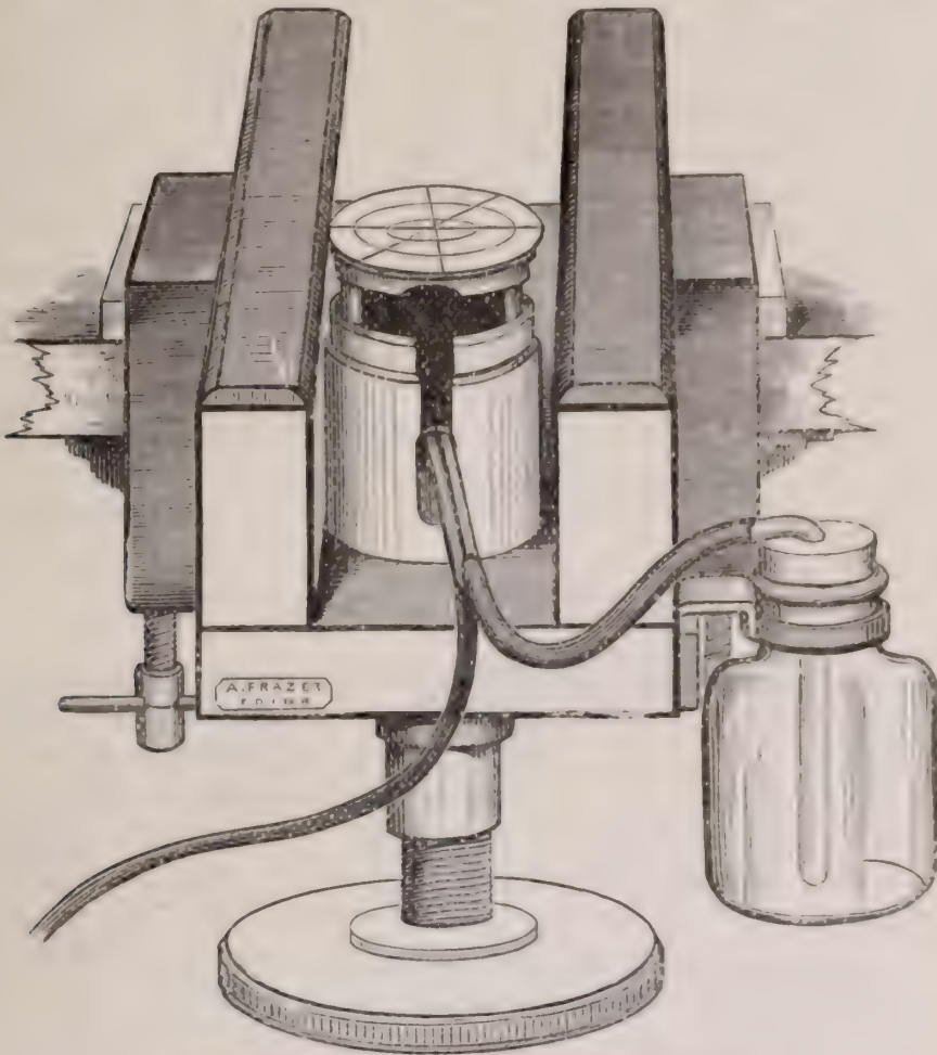
FIG. 355.—Catheart's freezing microtome.
