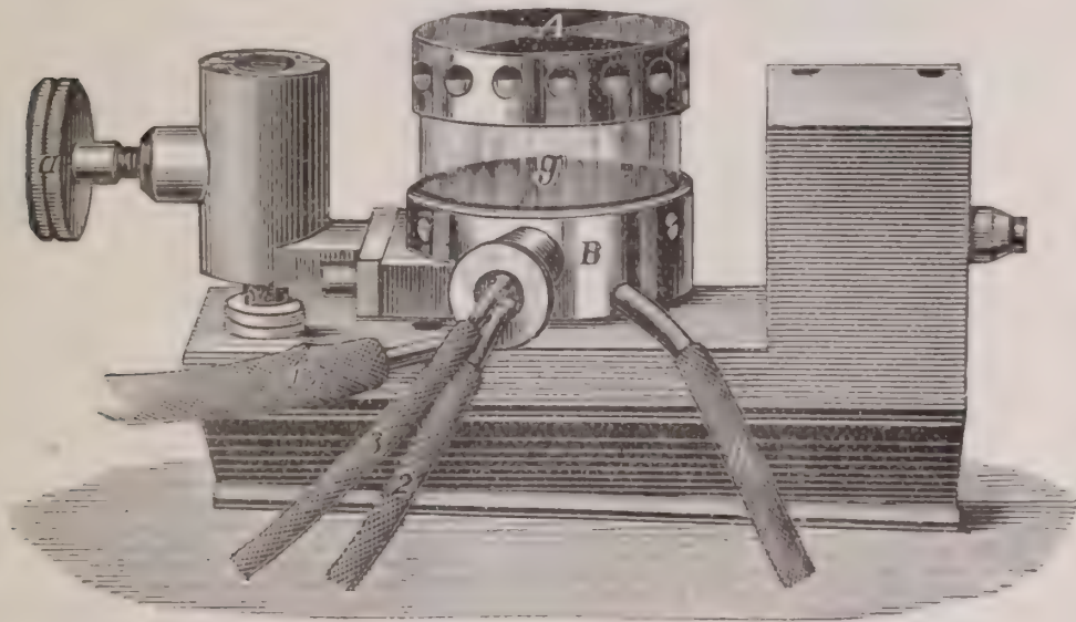
FIG. 350.—Freezing apparatus for the Thoma microtome.
