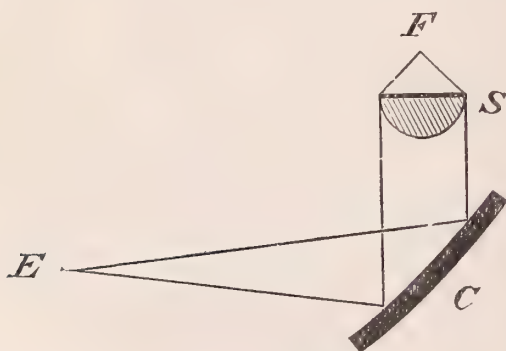
FIG. 309.—Same result with concave mirror.
